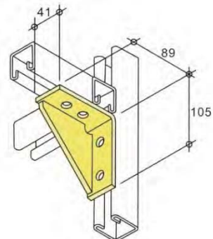
LH1332 - weight 432g
