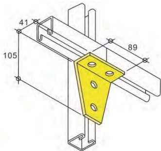
LH1359 - weight 458g
