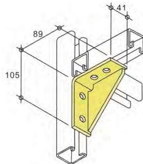
LH1331 - weight 432g
