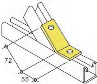
LH1546-45° - weight 243g
