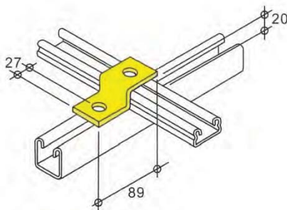
LH4045 - weight 180g
