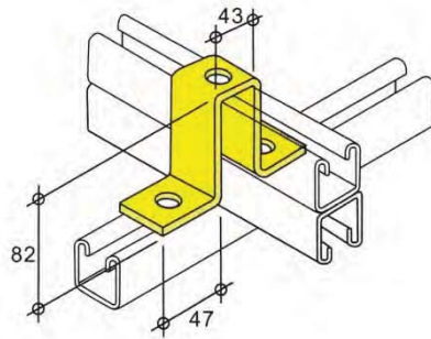
LH1737 - weight 530g
