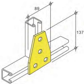
LH1358 - weight 450g
