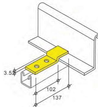
LHZB04 - weight 251g
