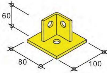
LH2072/S1 - weight 568g
