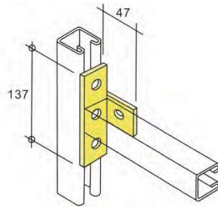
LH1033 - weight 342g
