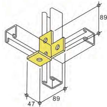
LH1035 - weight 342g
