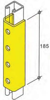
LH1377 - weight 1109g
