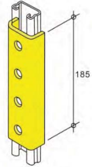
LH4377 - weight 760g
