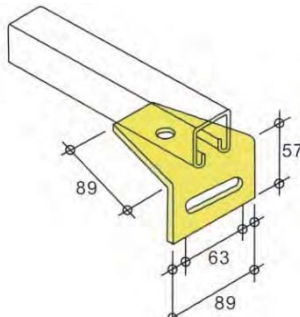
LH1713 - weight 384g
