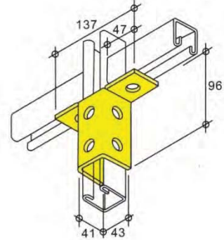
LH2346 - weight 726g
