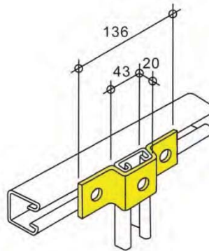
LH4047 - weight 284g
