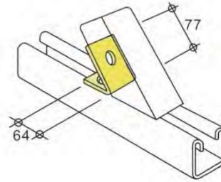
LH1186-45° - weight 256g
