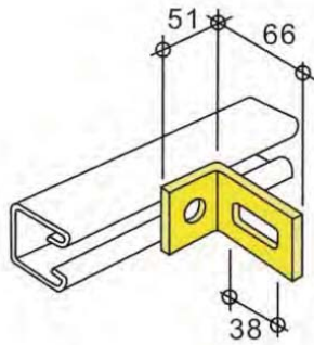
LH1749 - weight 194g
