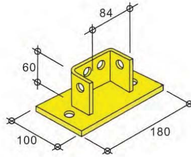
LH2073/A - weight 1927g
