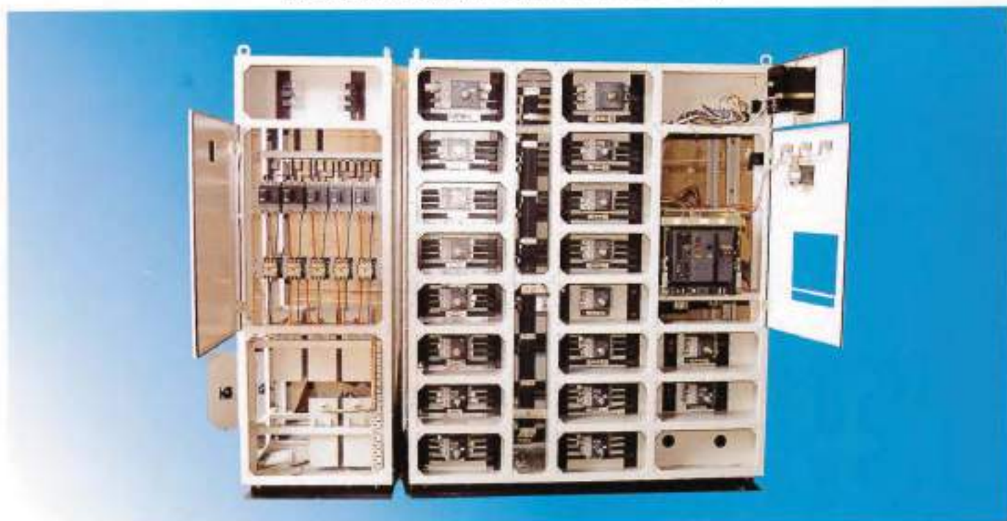
工廠車間總配電櫃 (加裝自動補償器) Main Power Supply Panel(With Capacitor Bank)
