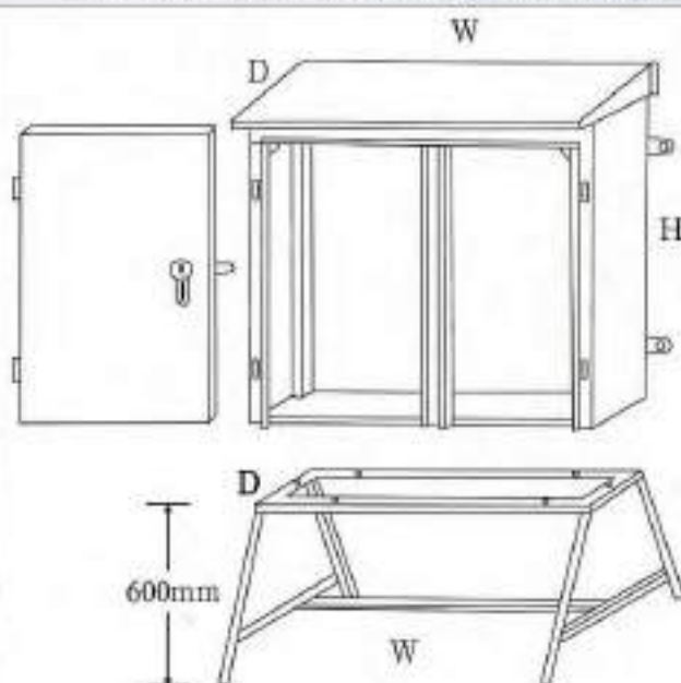
露天用避水箱結構圖 Structural diagram of outdoor waterproof panel
